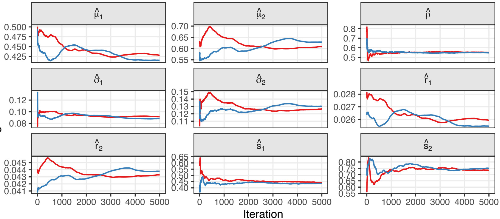
Ergodic mean
