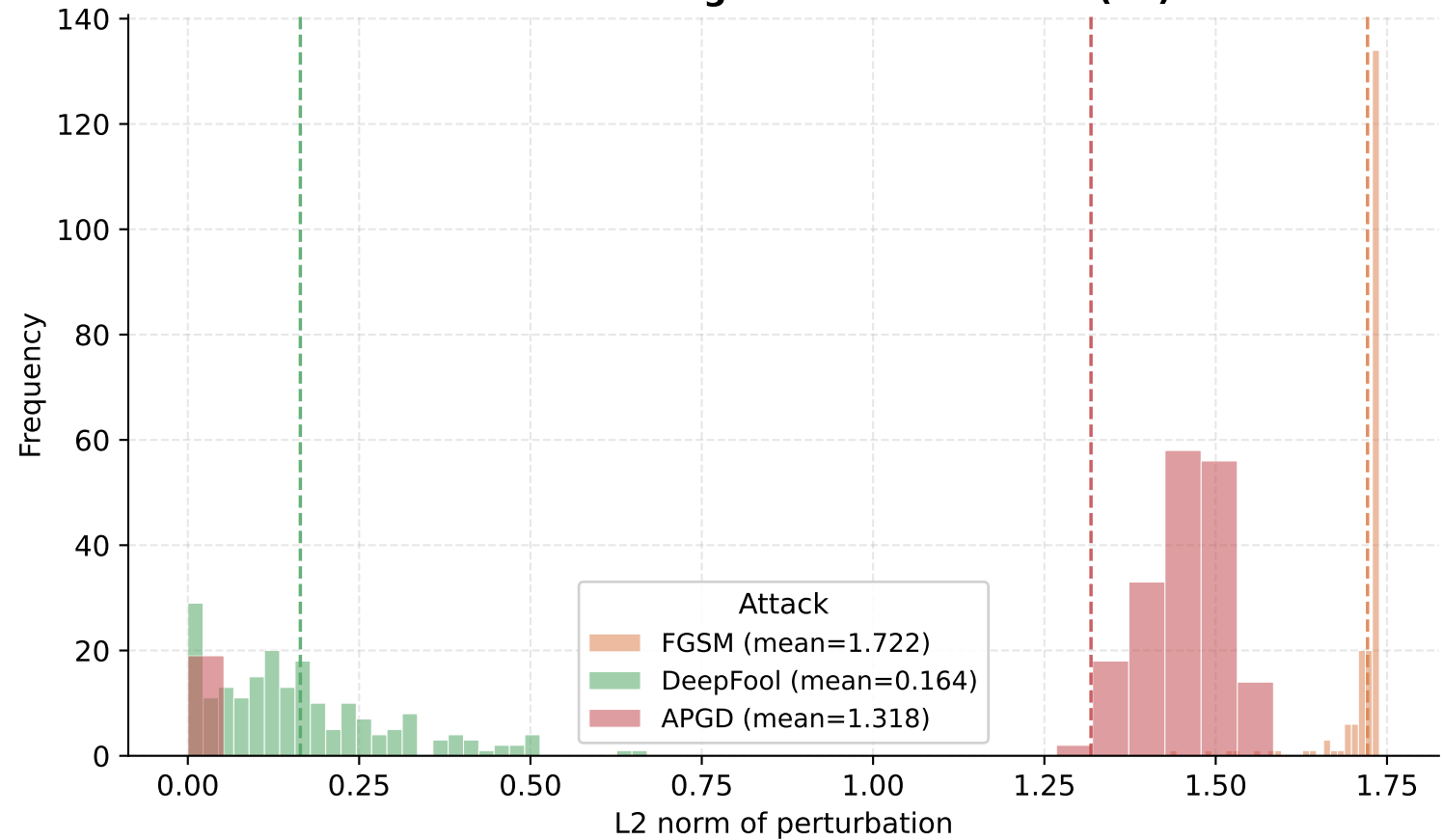
Perturbation Magnitude Distribution (L2)
