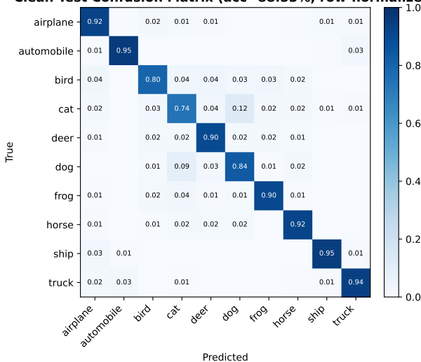
Clean Test Confusion Matrix (acc=88.53%, row-normalized)
