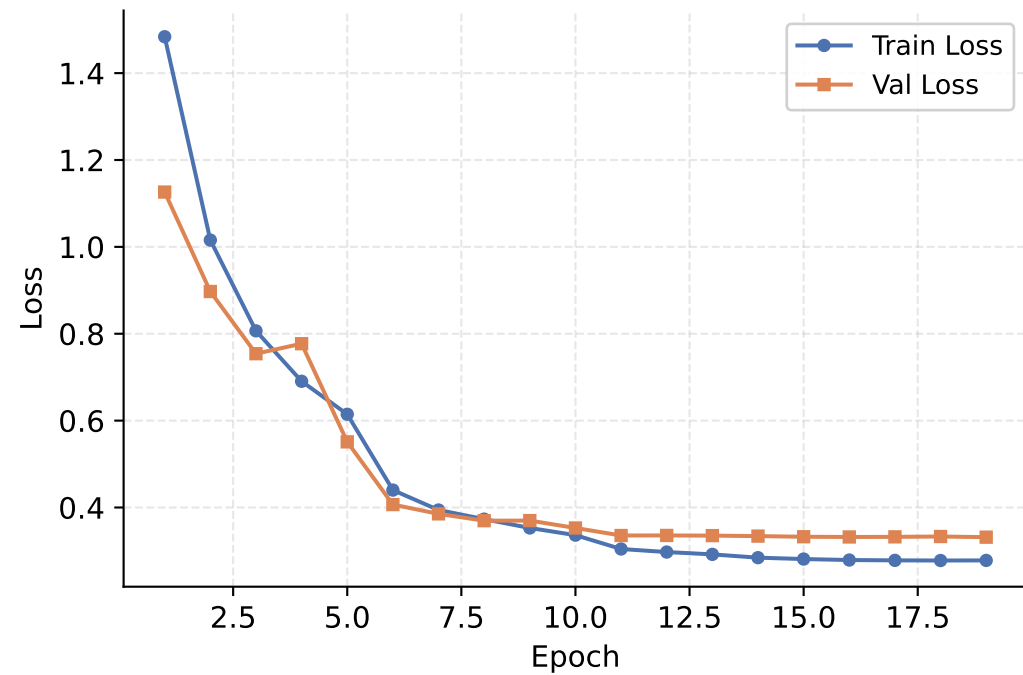
Loss Curves
