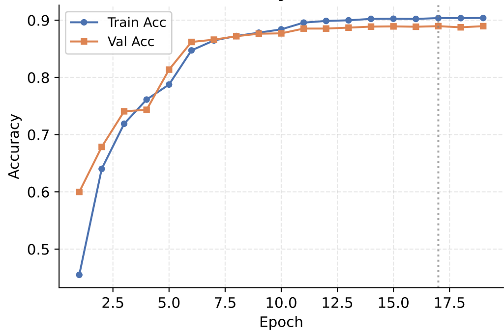
Accuracy Curves
