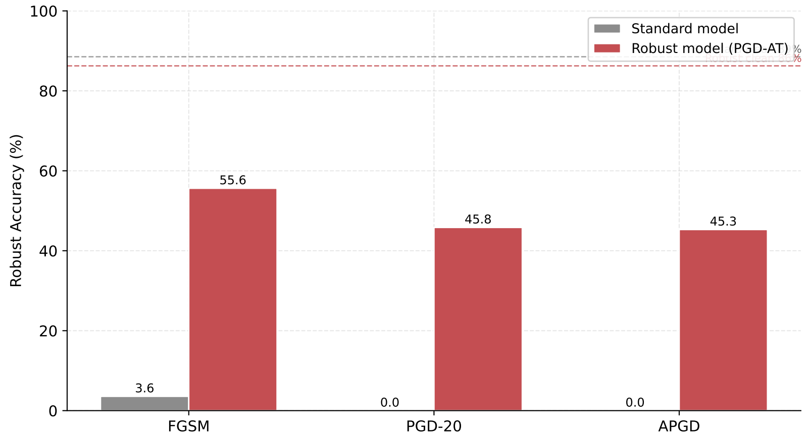
Robust Accuracy vs Attack Strength (FGSM < PGD-20 < APGD)
