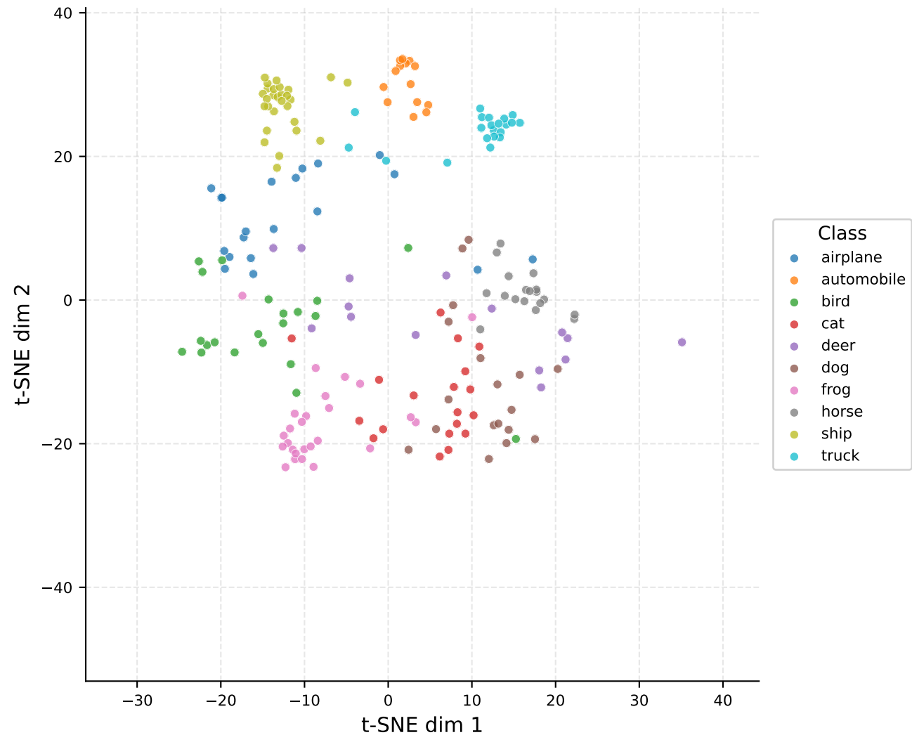
t-SNE: Clean (by class)
