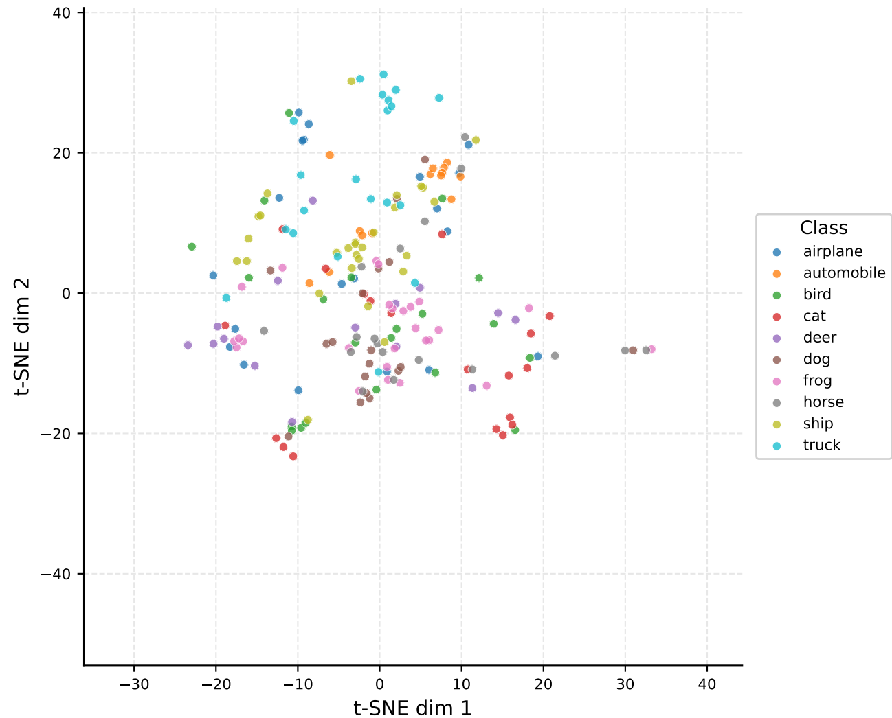
t-SNE: FGSM (by class)
