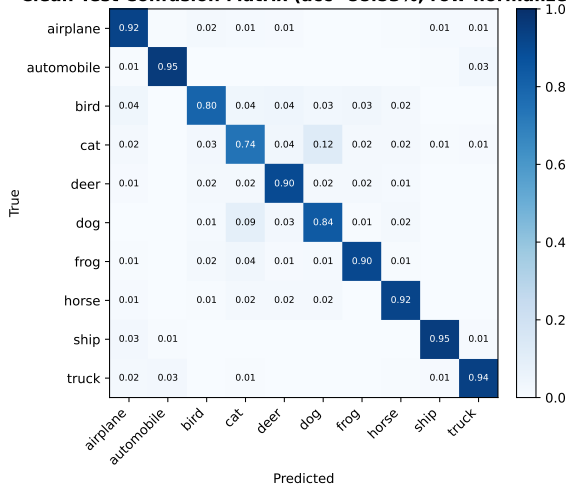
Clean Test Confusion Matrix (acc=88.53%, row-normalized)
