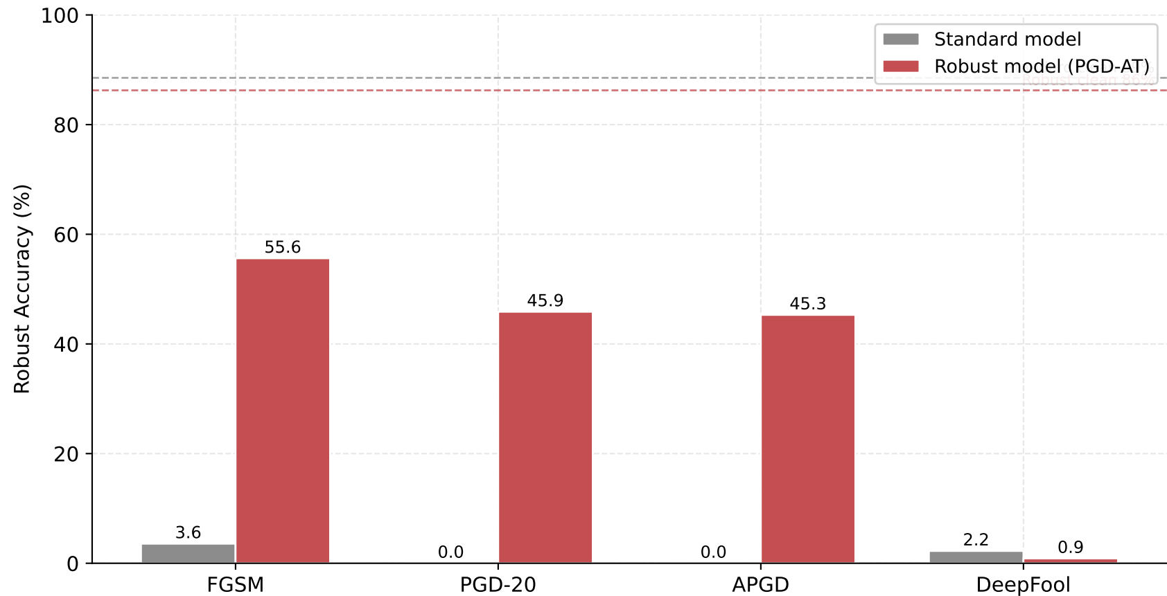
Robust Accuracy: Standard vs Robust (FGSM / PGD-20 / APGD / DeepFool)
