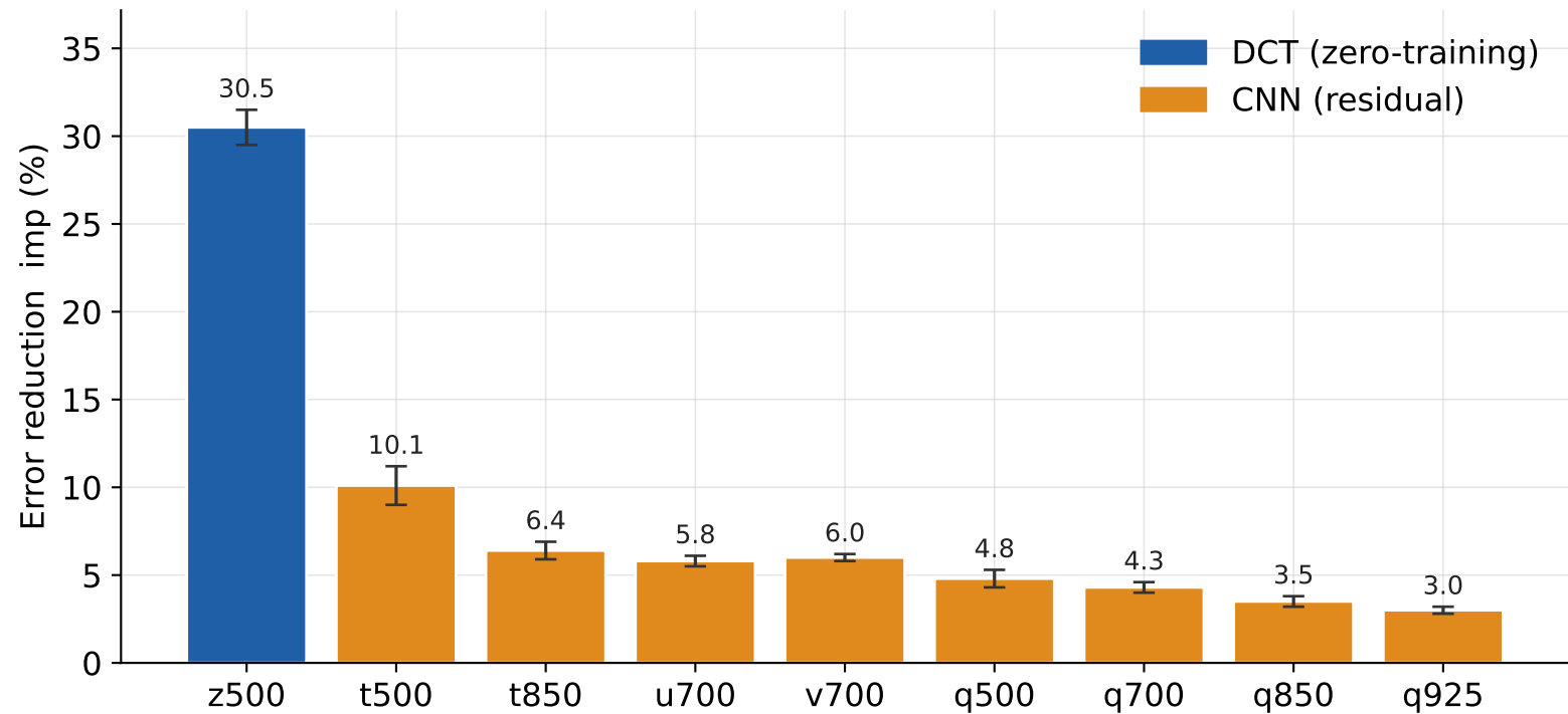
Assimilation skill: zero-training DCT (large-scale) + lightweight CNN
