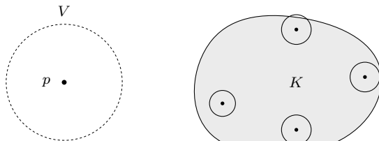
W: finitely many balls covering K
