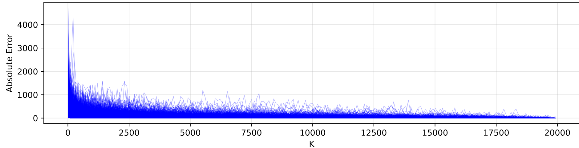
Absolute Error vs K
