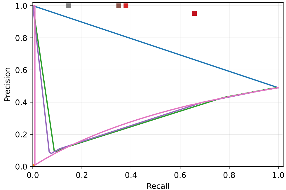
safelawbench: PR
