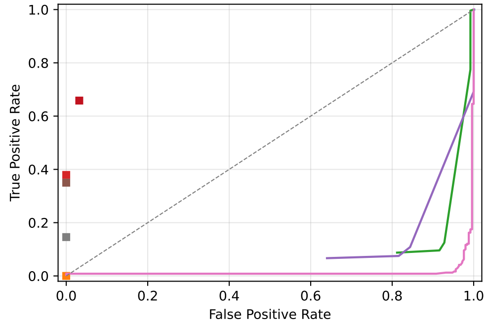
safelawbench: ROC
