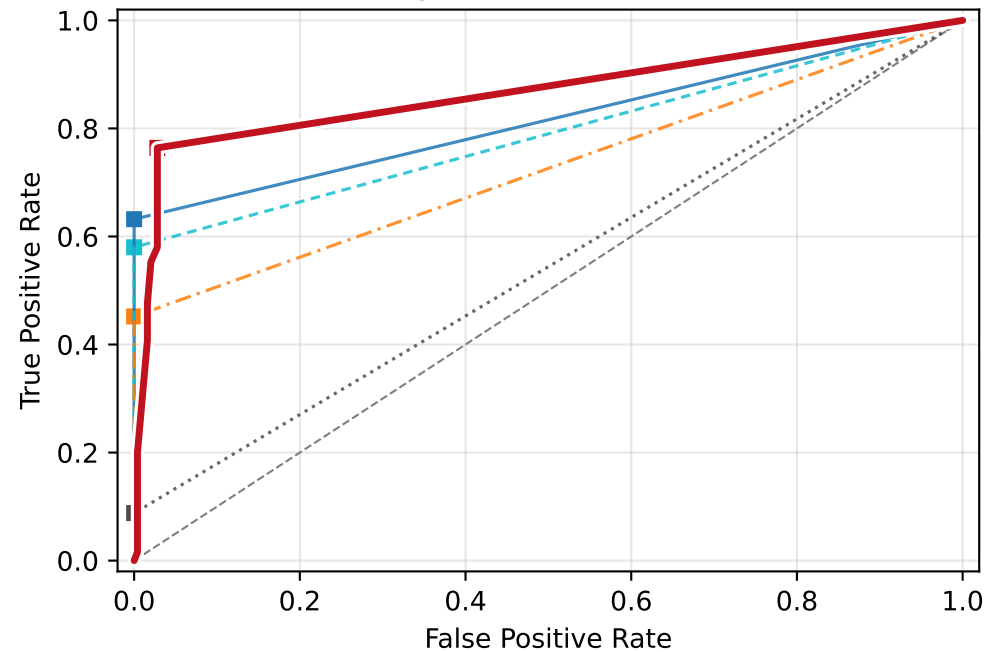
agentdefense: ROC
