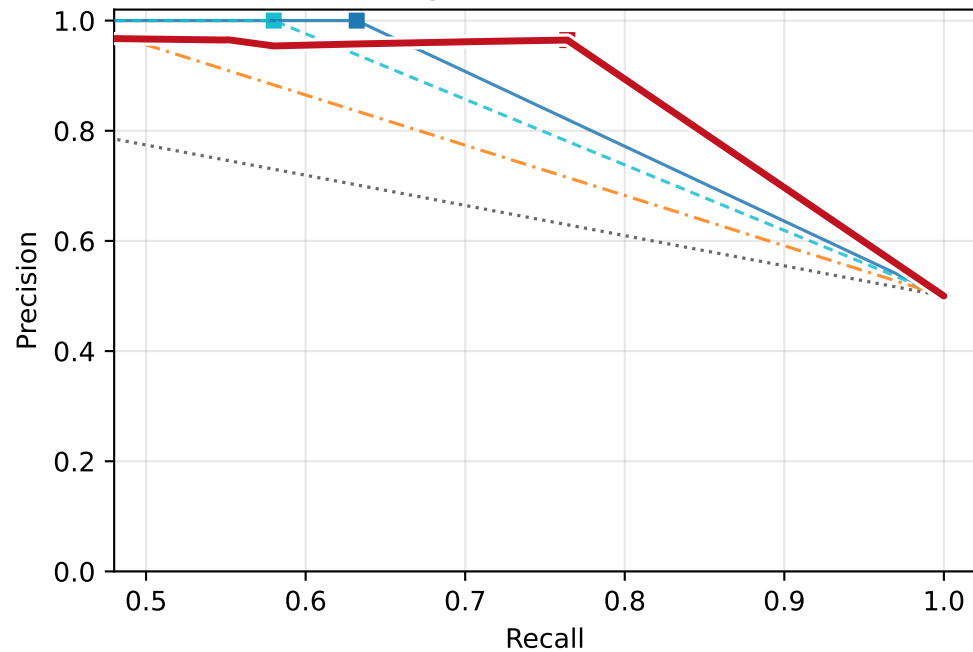
agentdefense: PR
