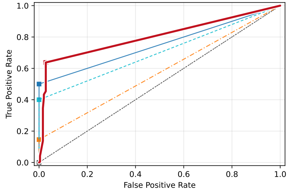
safeclawbench: ROC
