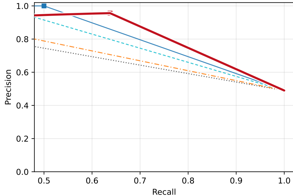
safeclawbench: PR
