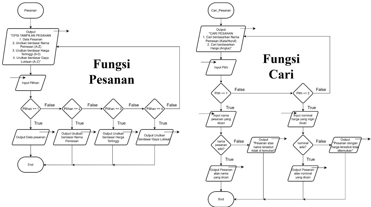
Gambar Flowchart 1.4
