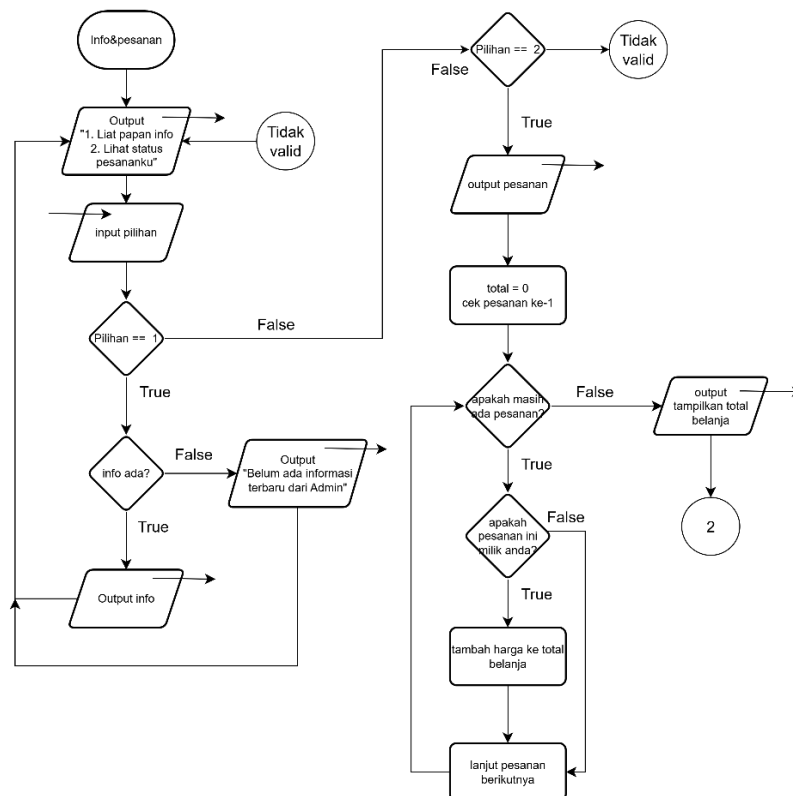
Gambar Flowchart 1.5
