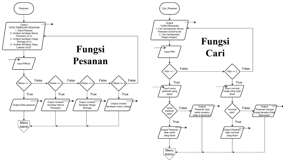
Gambar Flowchart 1.4
