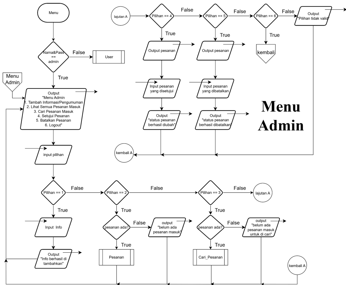
Gambar Flowchart 1.3
