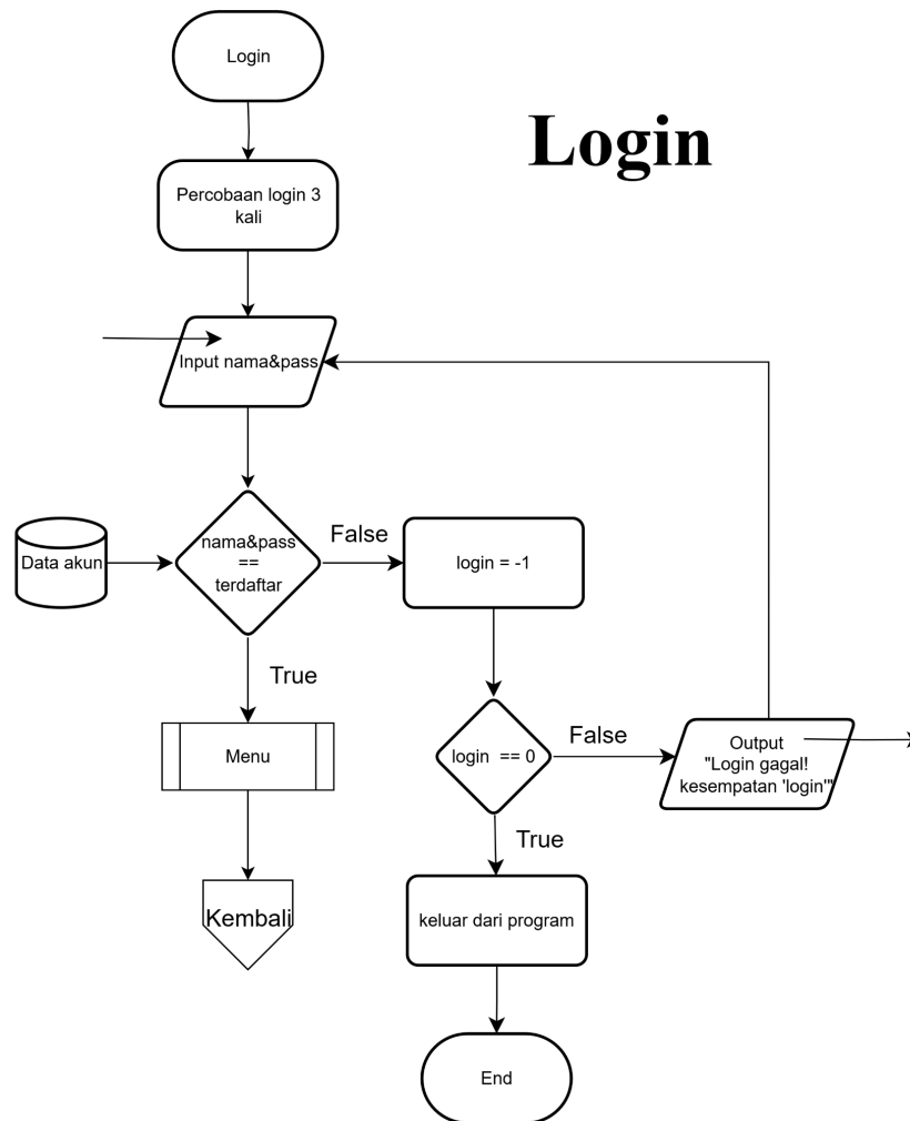
Gambar Flowchart 1.2
