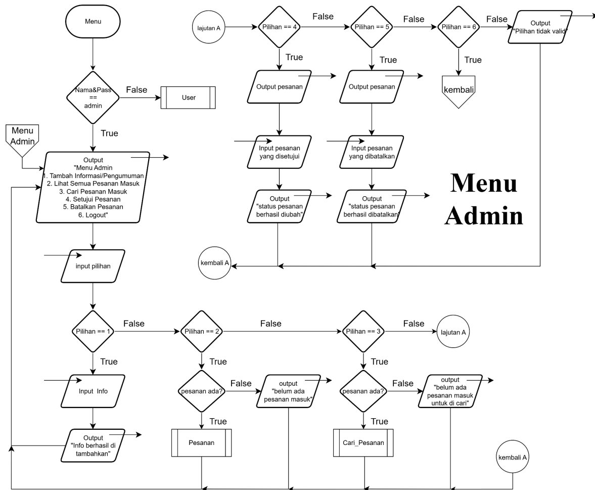
Gambar Flowchart 1.3
