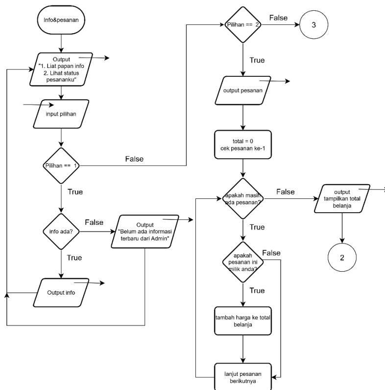
Gambar Flowchart 1.5
