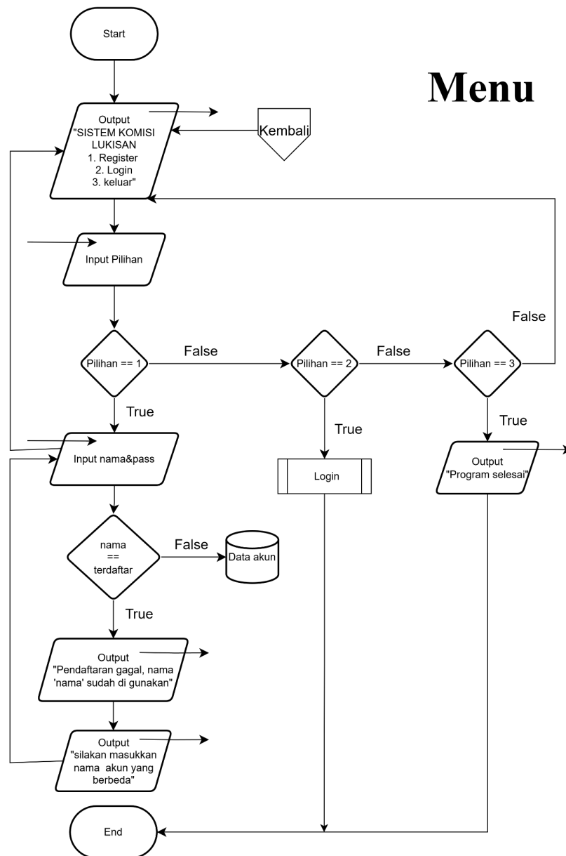
Gambar Flowchart 1.1
