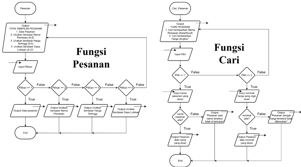
Gambar Flowchart 1.4
