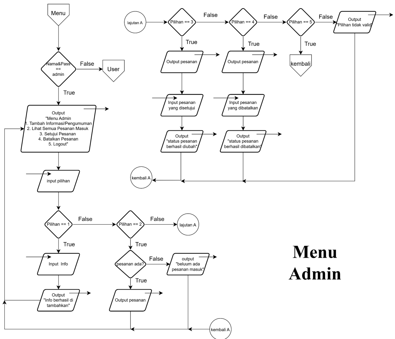
Gambar Flowchart 1.3
