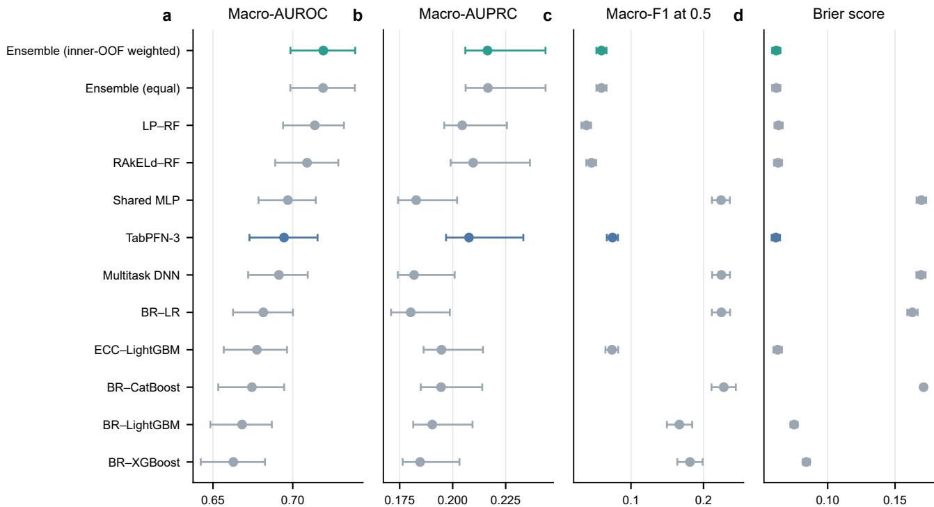
Repeated outer-fold performance with 95% patient-bootstrap intervals
