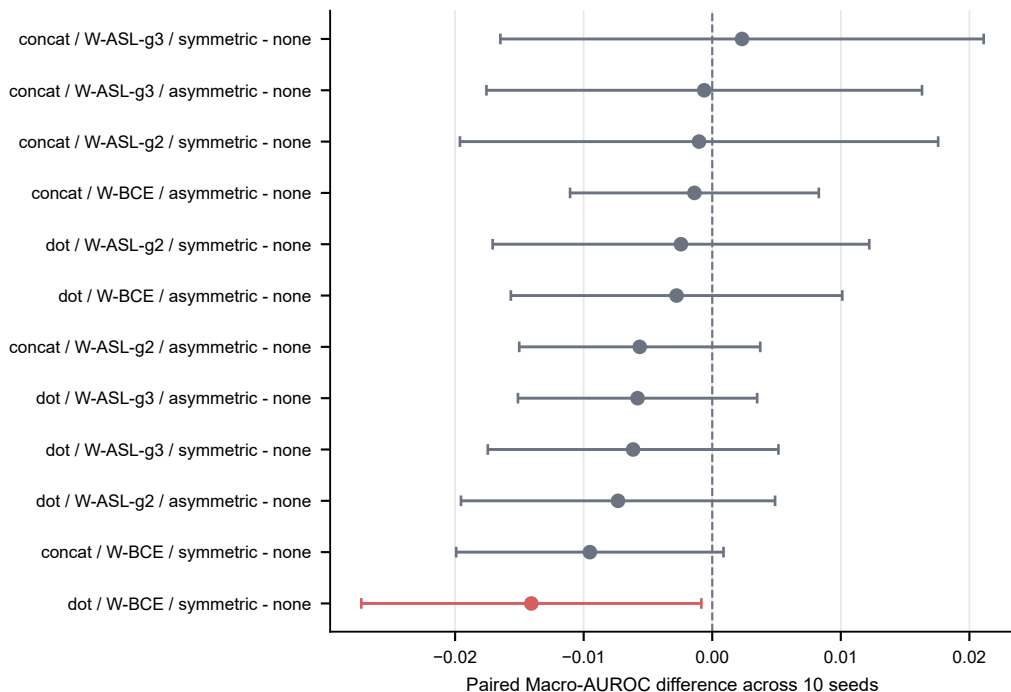
Graph variants relative to matched no-graph controls
