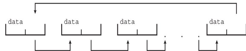
Circularly linked list
