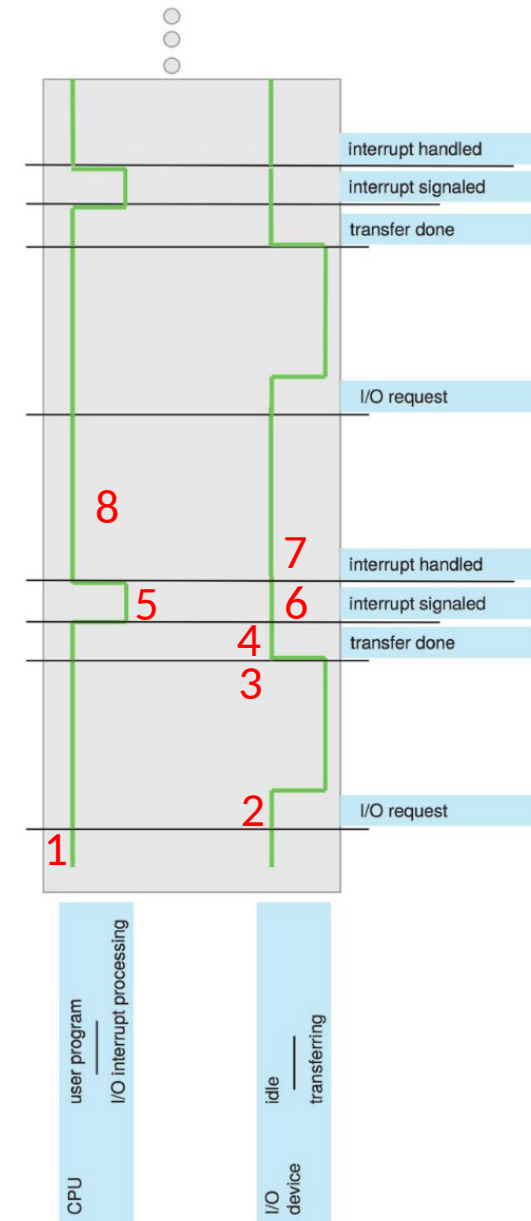
Interrupt timeline for a single program doing output
