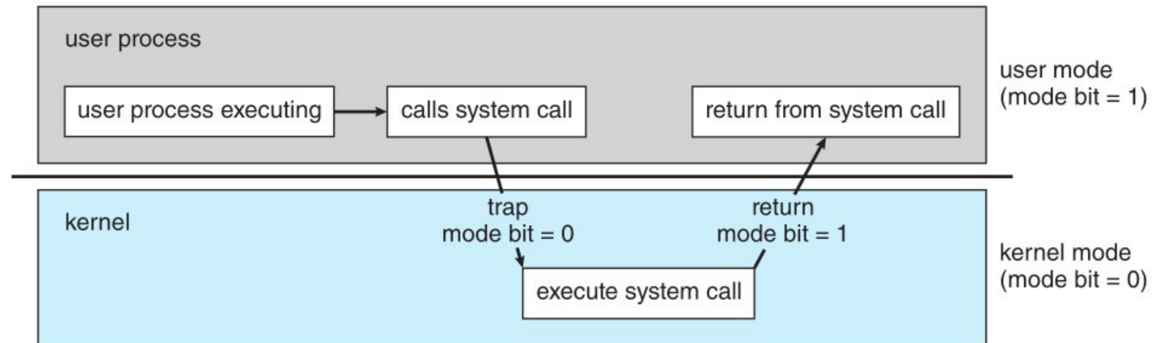
Transition from user to kernel mode.
