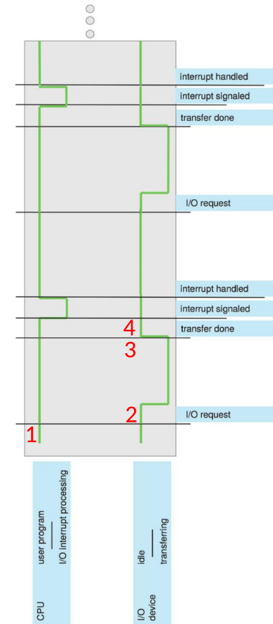
Interrupt timeline for a single program doing output
