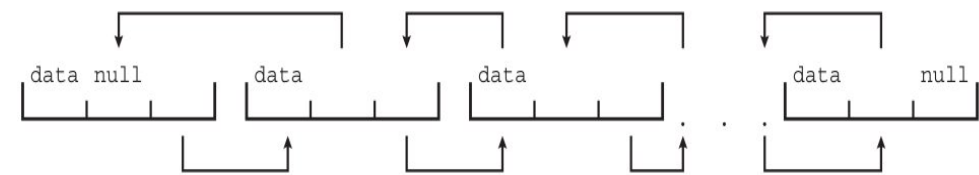
Doubly linked list
