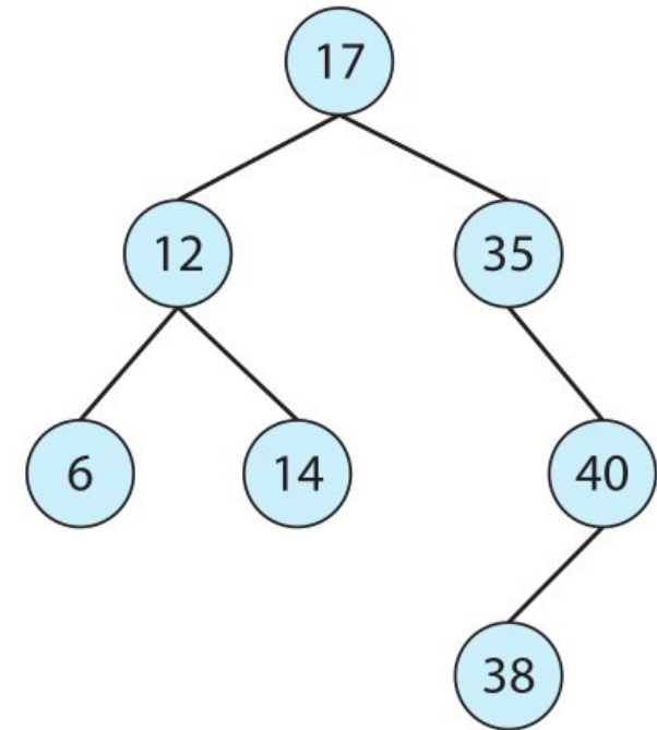
binary search tree
