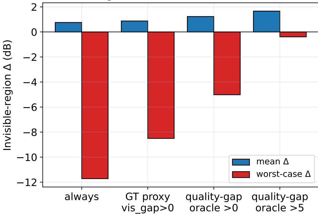
Oracle diagnostic: mean vs worst-case (N=166)
