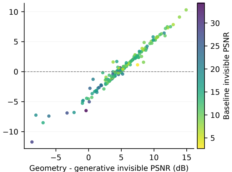
(a) Evidence gap predicts benefit r = 0.982 , N = 166
