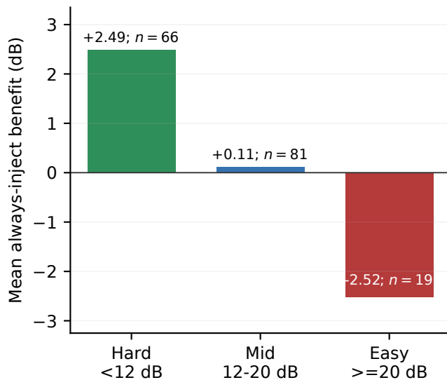
(b) Benefit depends on baseline difficulty
