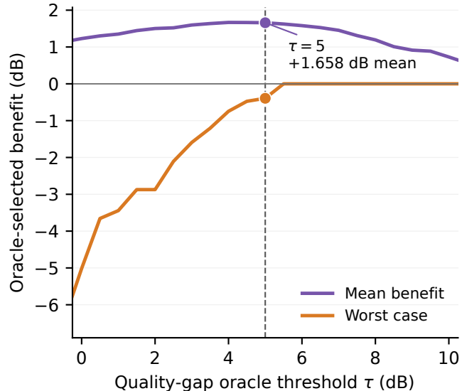
(c) Oracle selectivity Mean and worst-case benefit
