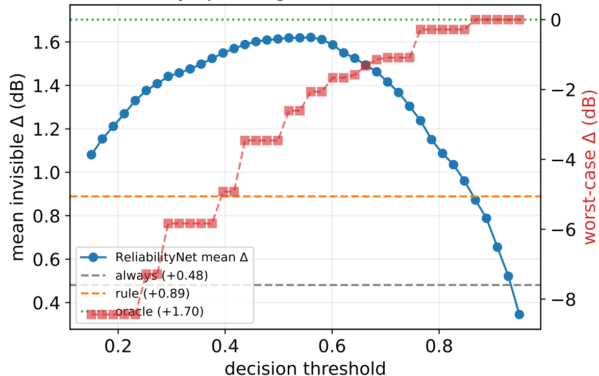
Reliability operating frontier (frames=2898)
