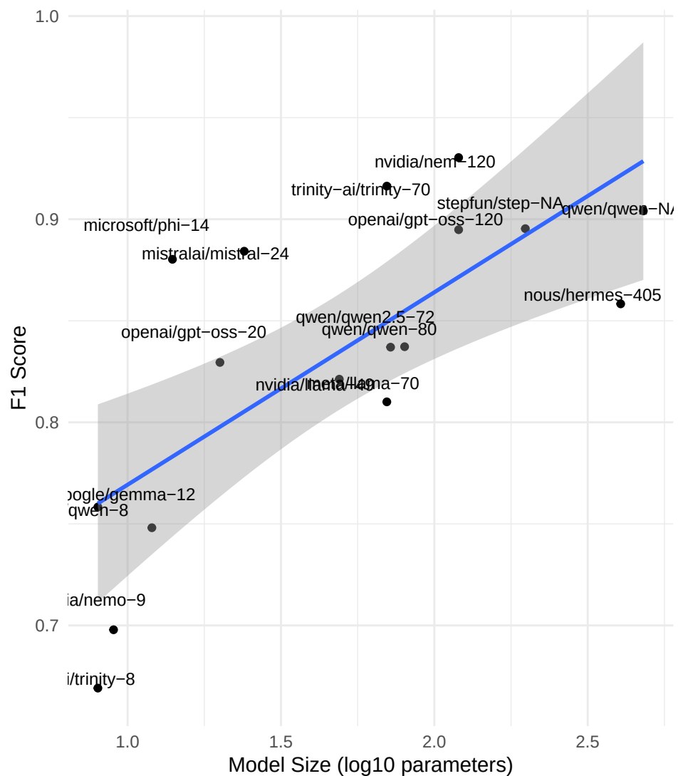
Effect of Model Size on F1 Score
