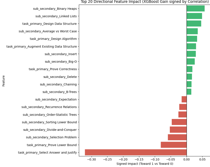
Figure 9. Directional feature importance based on XGBoost gain values.
