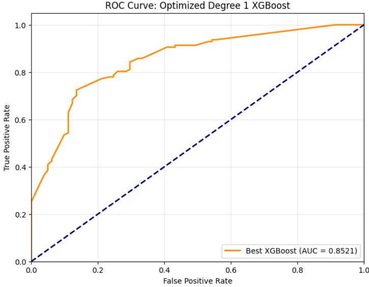
Figure 8. ROC curve for the optimized XGBoost classifier.
