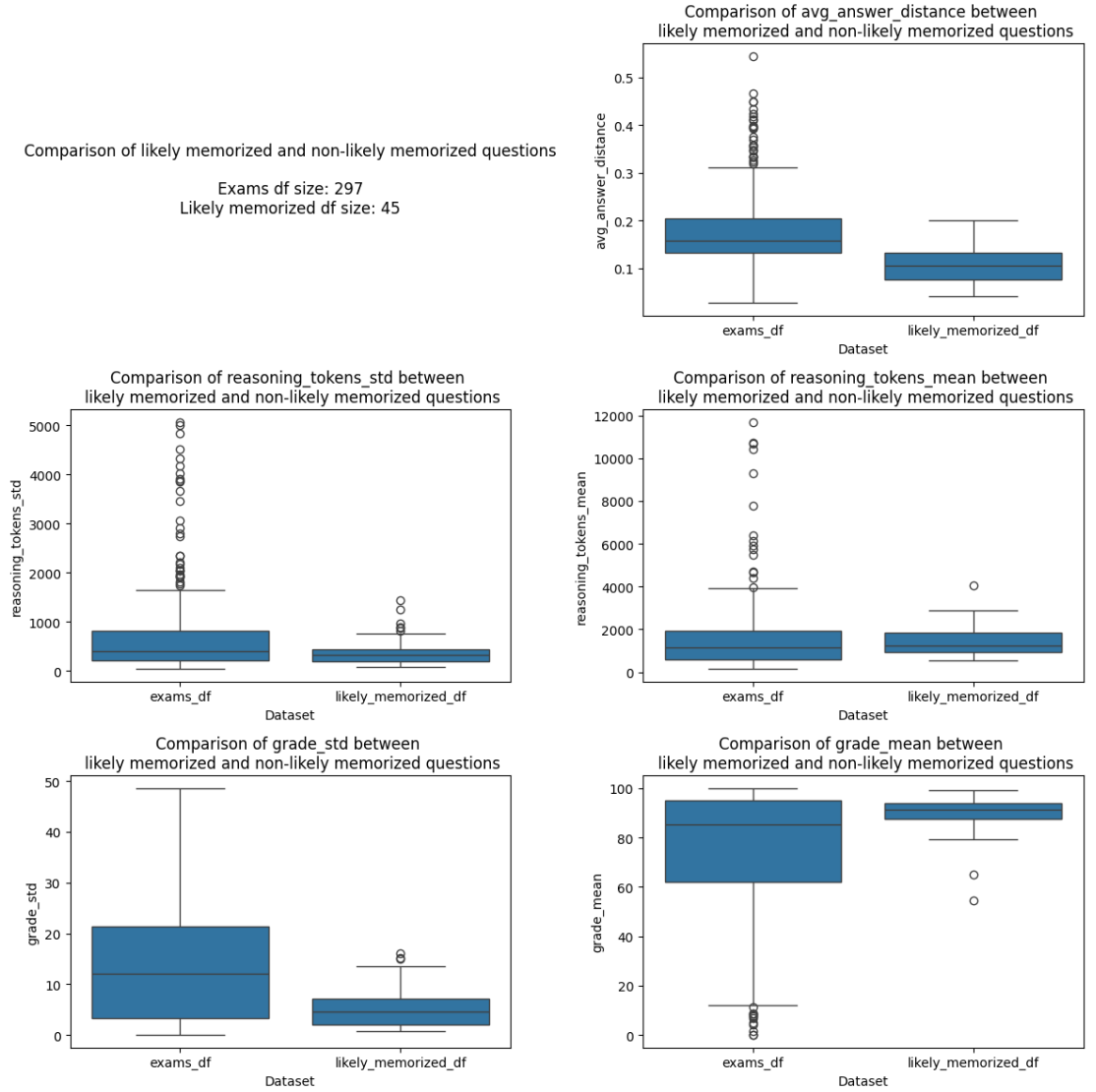
Figure 3. Comparison of output-variance metrics between the exam dataset and the likely memorized dataset.
