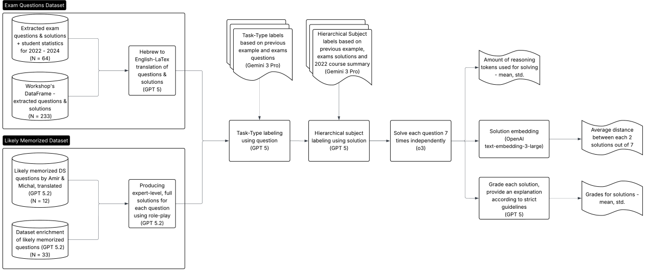
Figure 2. Dataset construction and metric extraction pipeline.
