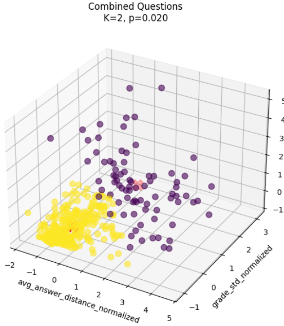
Figure 4. K-means clustering of questions in the normalized metric space.
