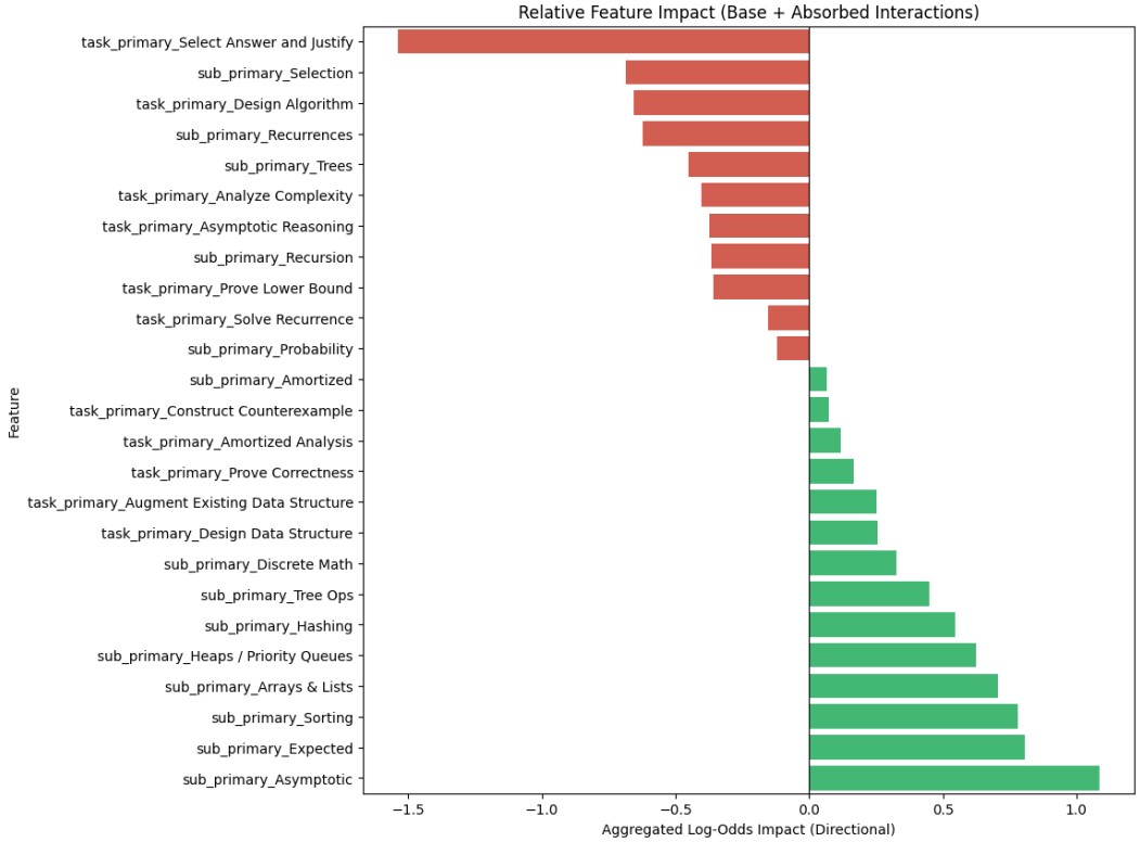
Figure 6. Relative feature impact in the logistic regression model, including both direct and interaction effects.
