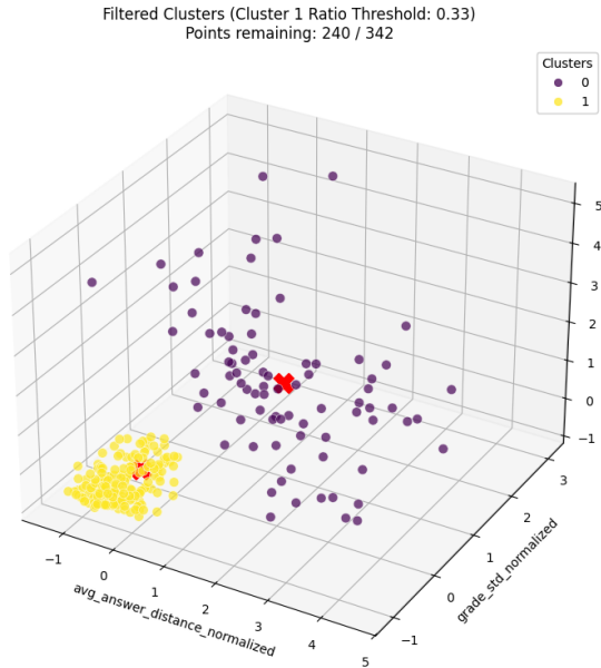
Figure 5. Filtered question set after removing borderline samples based on the distance ratio threshold.
