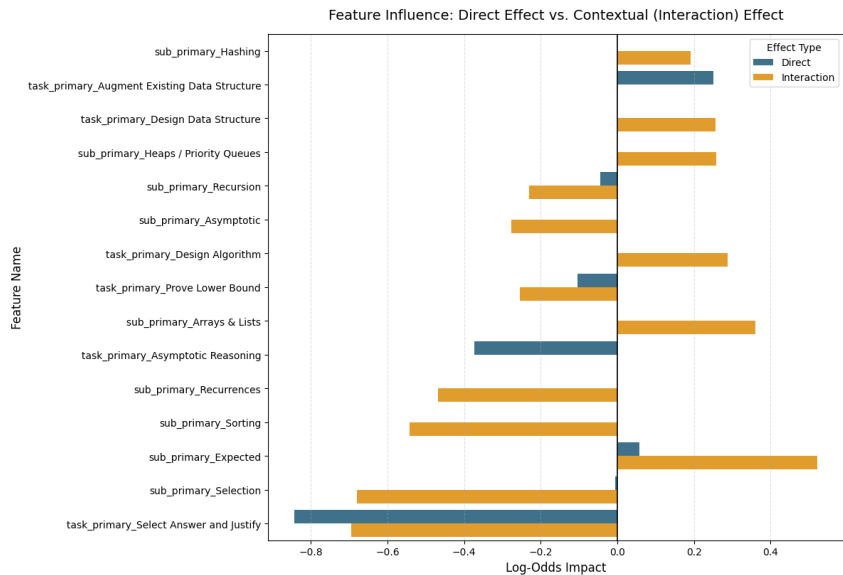
Figure 7. Direct feature effects versus contextual interaction effects in the logistic regression model.
