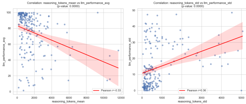
Figure 12. Relationship between reasoning token usage and model performance. Left: correlation between reasoning token mean and average grade. Right: correlation between reasoning token standard deviation and grade standard deviation.
