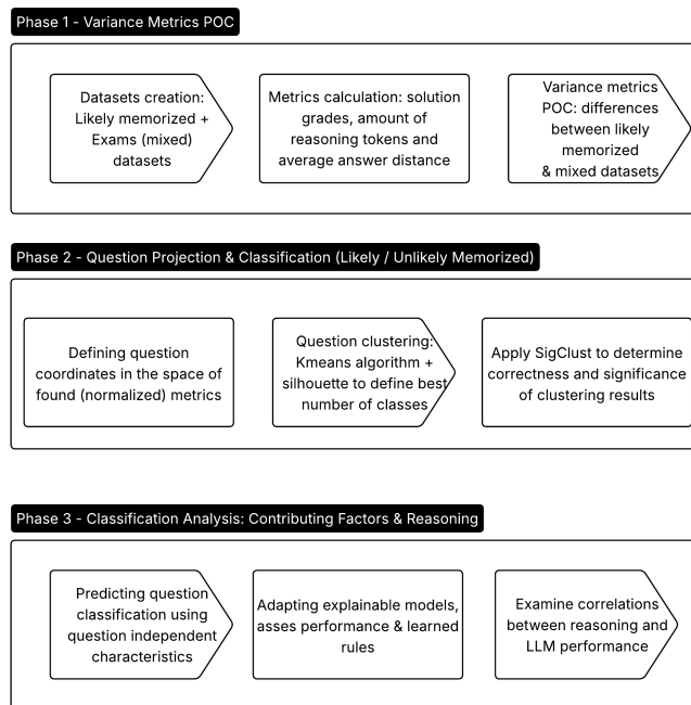
Figure 1. A three-phase pipeline for assessing LLM memorization in Data Structures and Algorithms questions: metric validation, clustering-based classification, and predictive analysis.
