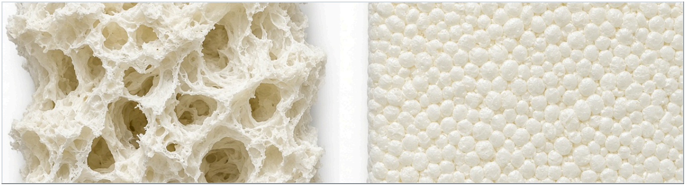
Left: open cell — windows broken, air passes, foam stays soft. Right: closed cell — membranes intact, gas trapped, foam is rigid and insulating.
