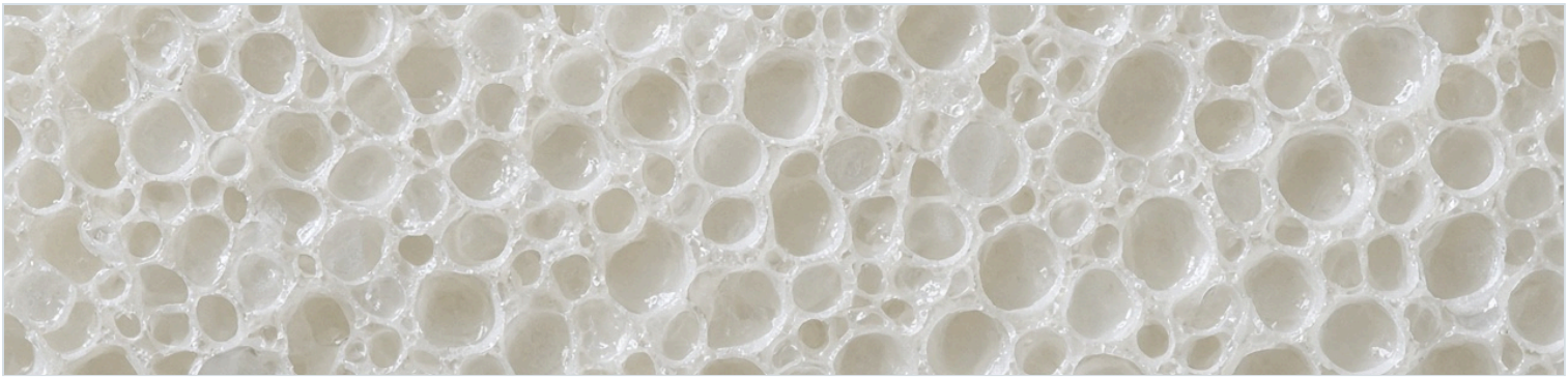
Closed-cell structure. Low water, higher index, and gel-heavy catalyst keep the membranes intact.
