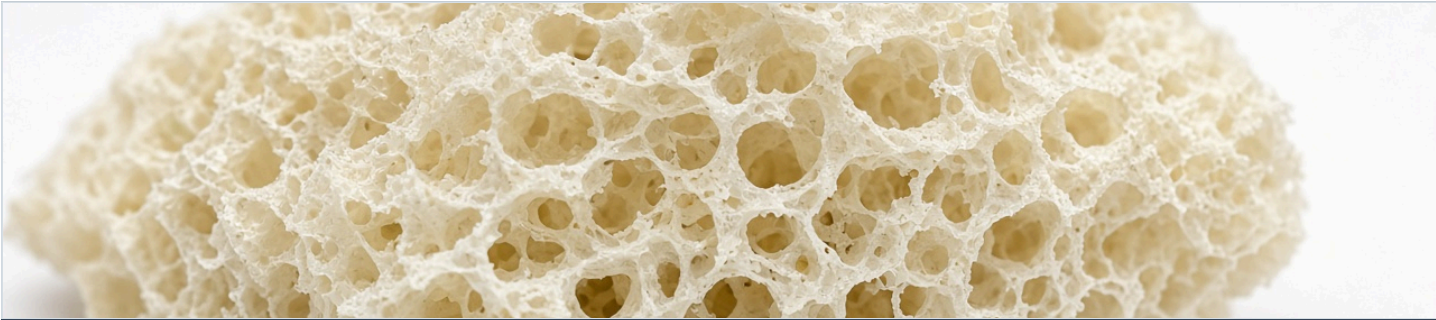
Open-cell structure. High water makes CO 2 . Catalysts blow faster than they gel so the windows rupture.
