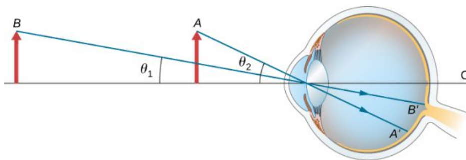
Figure 2.36 Size perceived by an eye is determined by the angle subtended by the object. An image formed on the retina by an object at A is larger than an image formed on the retina by the same object positioned at B (compared image heights OA' to OB' ).
