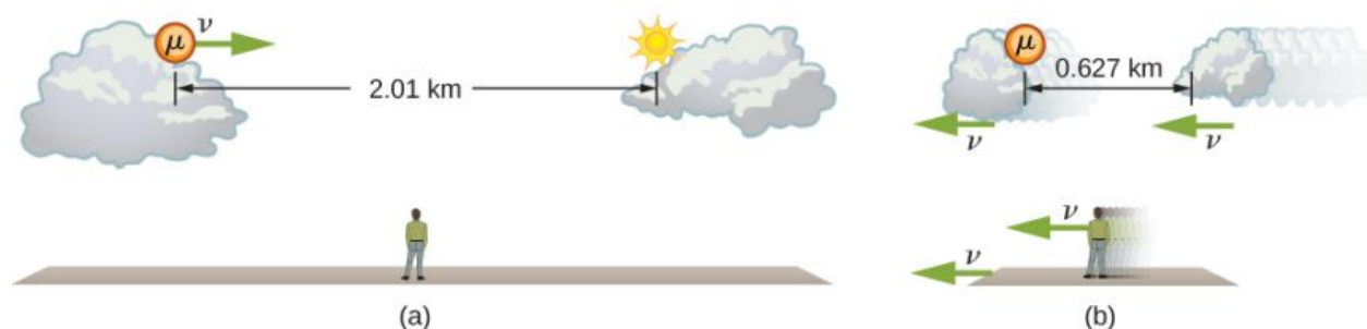
Figure 5.9 (a) The earthbound observer sees the muon travel 2.01 km. (b) The same path has length 0.627 km seen from the muon's frame of reference. The Earth, air, and clouds are moving relative to the muon in its frame, and have smaller lengths along the direction of travel.
