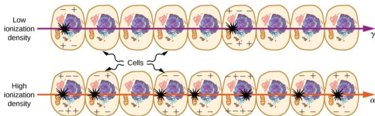
Figure 10.30 The image shows ionization created in cells by \alpha and \gamma radiation. Because of its shorter range, the ionization and damage created by \alpha rays is more concentrated and harder for the organism to repair. Thus, the RBE for \alpha rays is greater than the RBE for \gamma rays, even though they create the same amount of ionization at the same energy.
