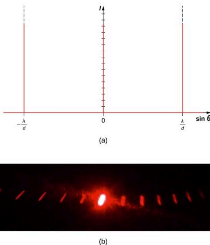
Figure 4.12 (a) Intensity of light transmitted through a large number of slits. When N approaches infinity, only the principal maxima remain as very bright and very narrow lines. (b) A laser beam passed through a diffraction grating. (credit b: modification of work by Sebastian Stapelberg)
