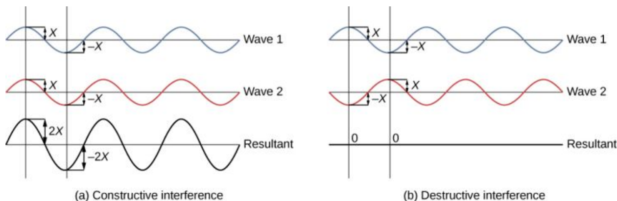
Figure 3.4 The amplitudes of waves add. (a) Pure constructive interference is obtained when identical waves are in phase. (b) Pure destructive interference occurs when identical waves are exactly out of phase, or shifted by half a wavelength.
