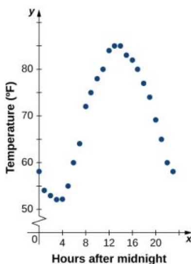
Figure 1.6 The graph of the data from Table 1.1 shows temperature as a function of time.
