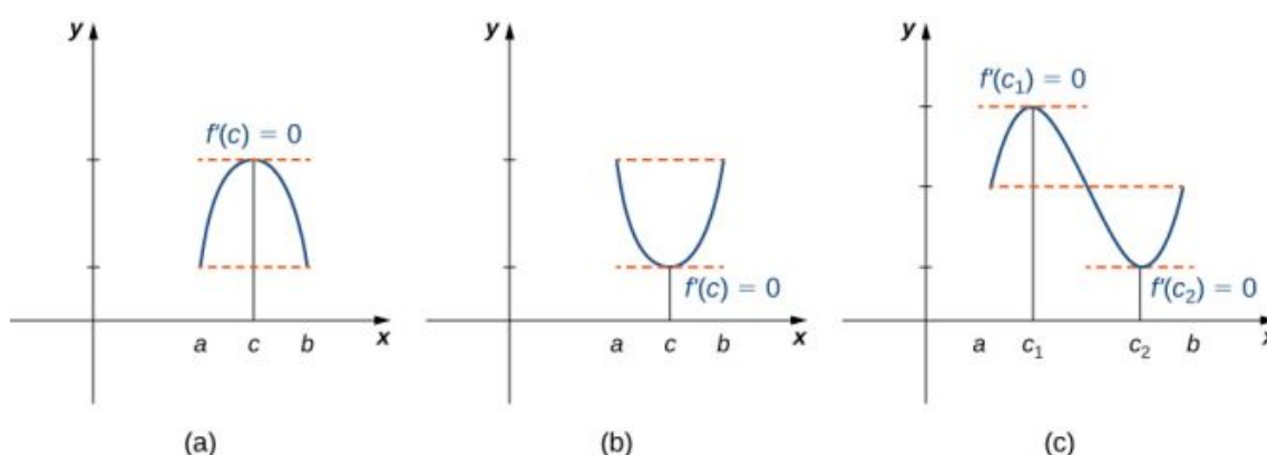
Figure 4.21 If a differentiable function f satisfies f(a) = f(b) , then its derivative must be zero at some point(s) between a and b .
