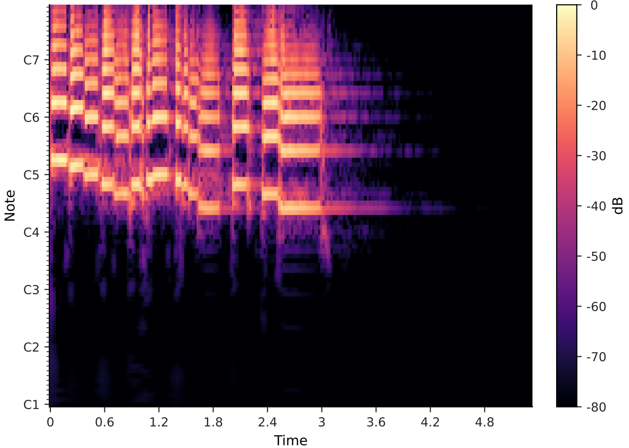
Constant-Q power spectrum
