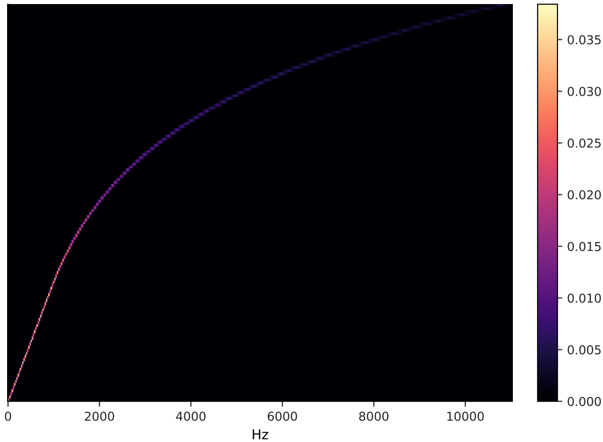
Mel filter bank
