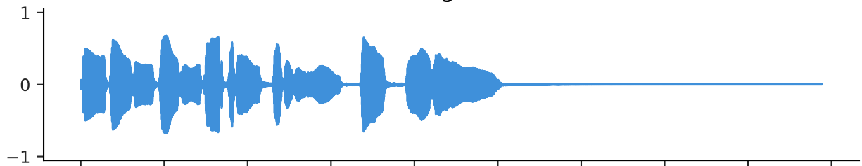
Griffin-Lim reconstruction
