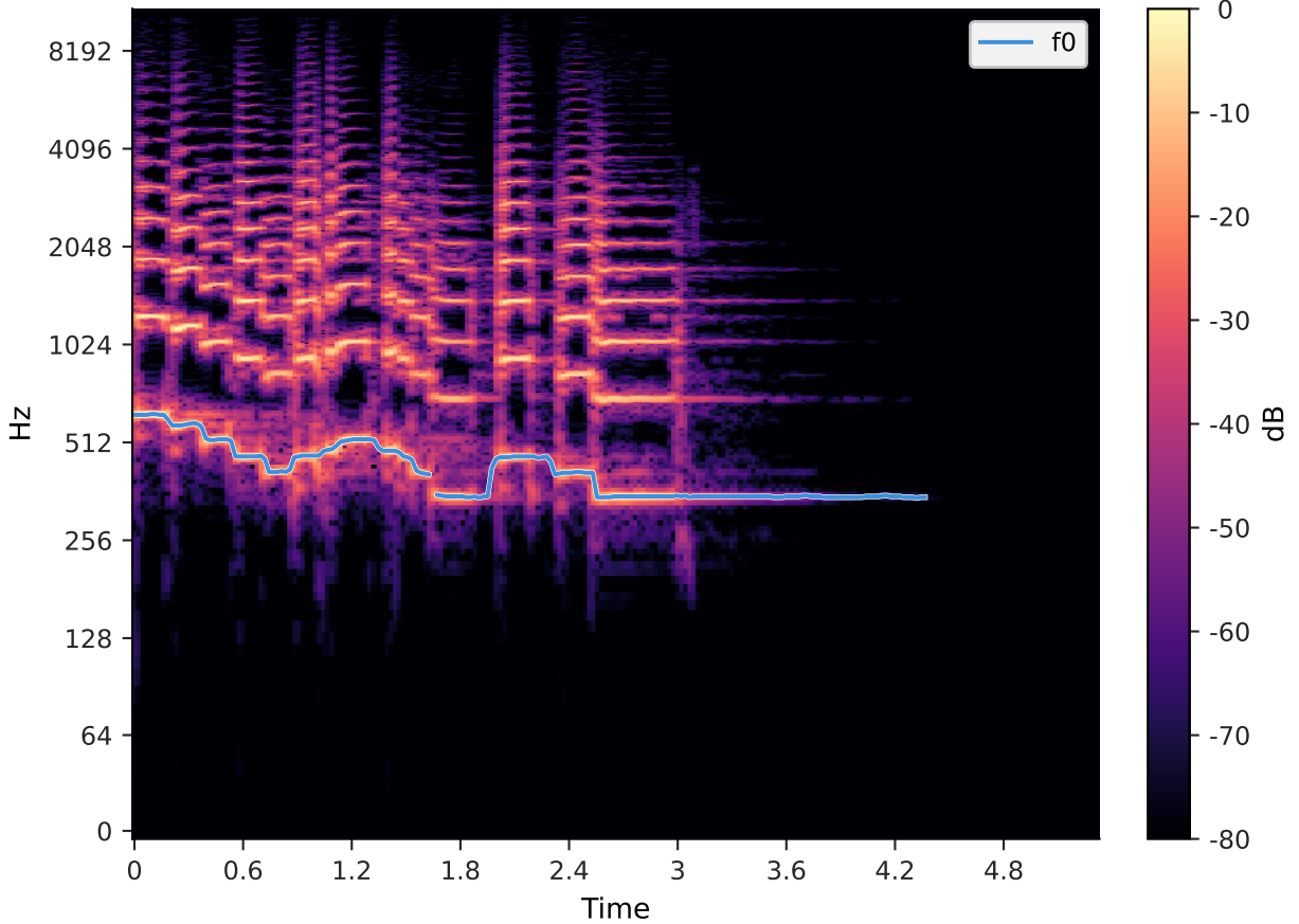
pYIN fundamental frequency estimation
