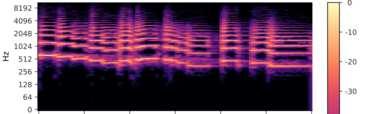
Salience spectrogram
