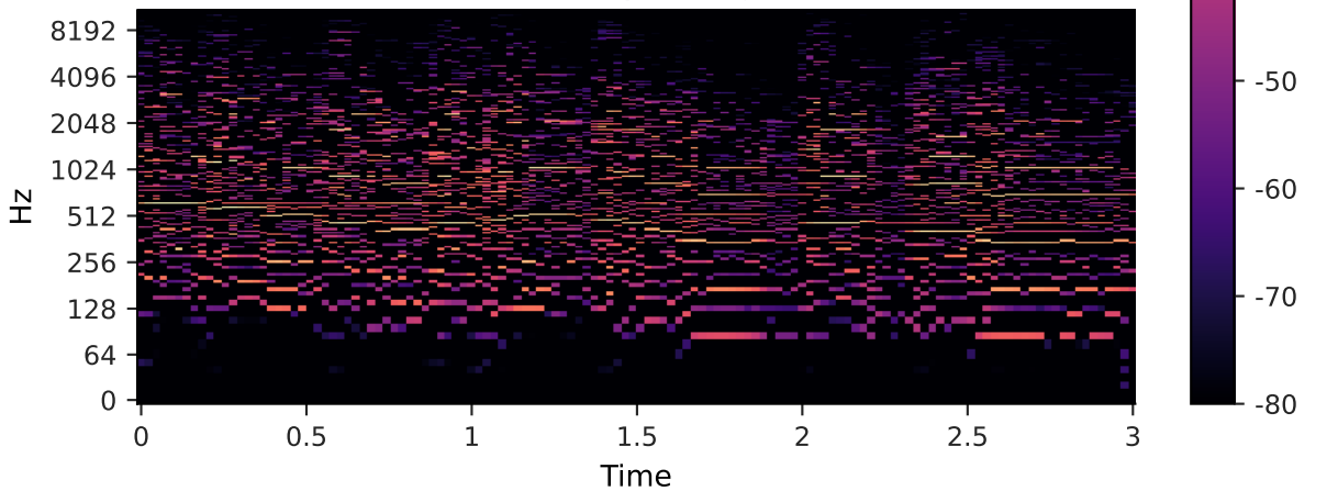
Salience spectrogram
