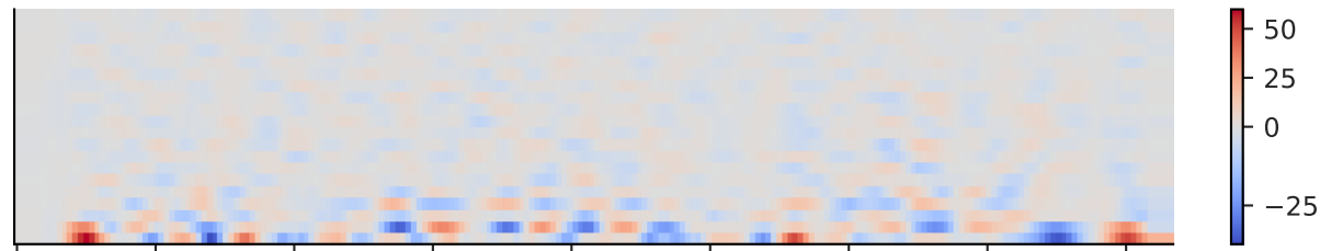
MFCC- \Delta^2
