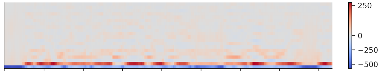
MFCC- \Delta
