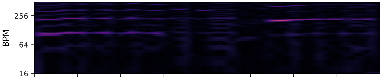
Autocorrelation tempogram
