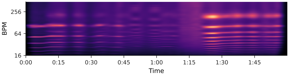
Autocorrelation tempogram
