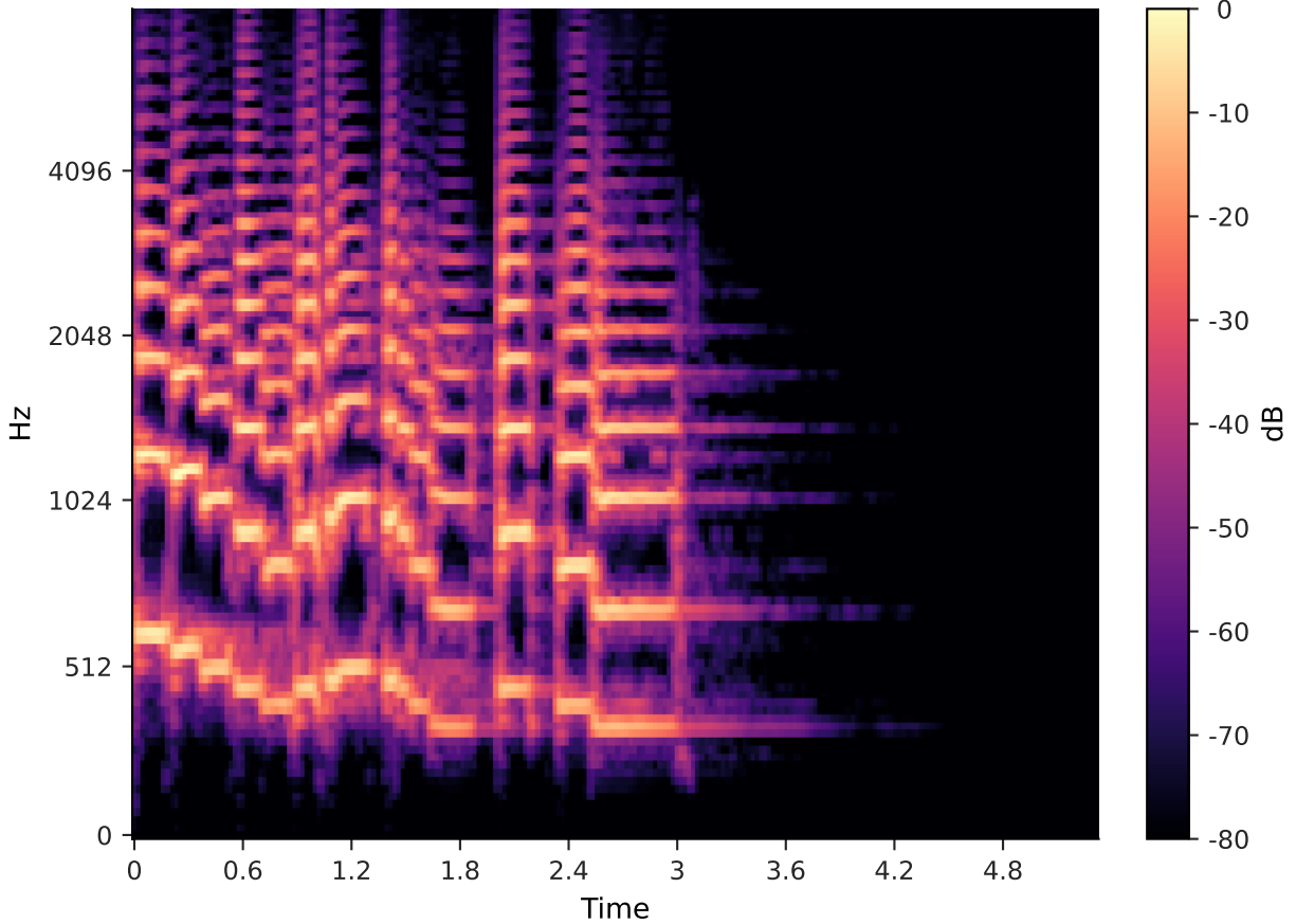
Mel-frequency spectrogram
