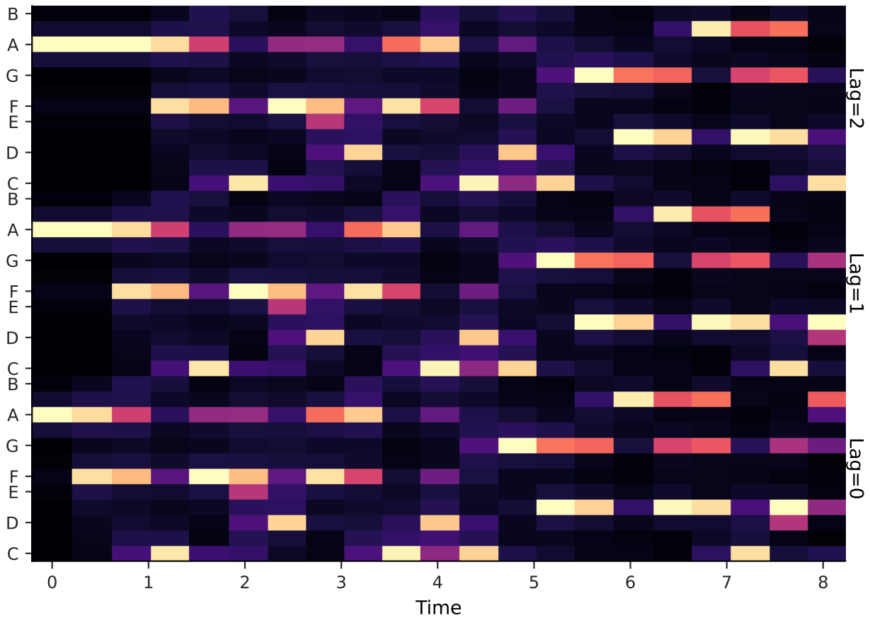
Time-lagged chroma
