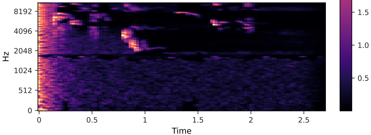
Per-channel energy normalization (max_size=3)
