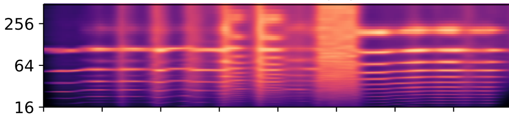
Fourier Tempogram
