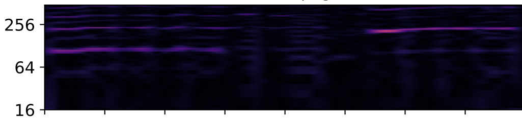
Hybrid Tempogram
