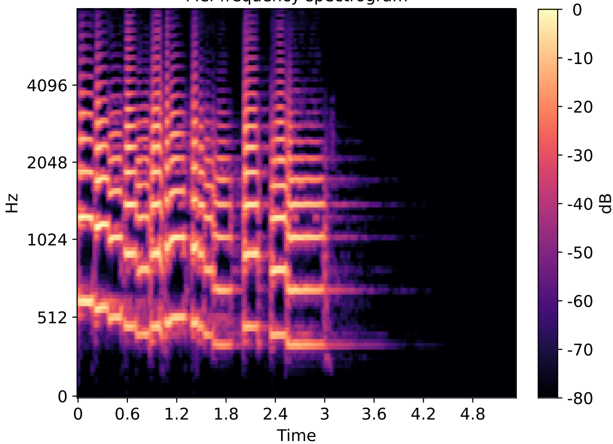
Mel-frequency spectrogram
