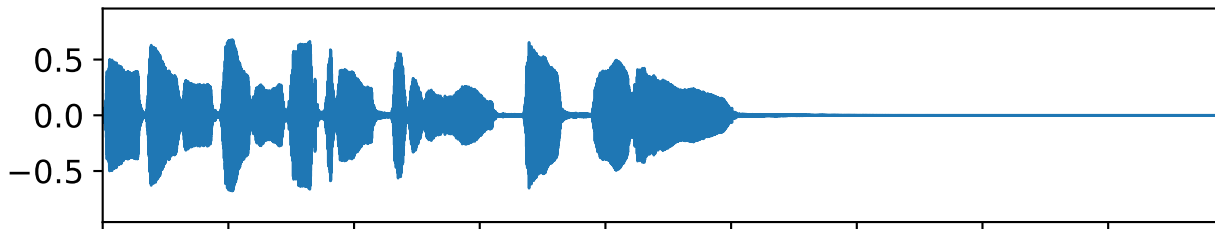
Griffin-Lim reconstruction
