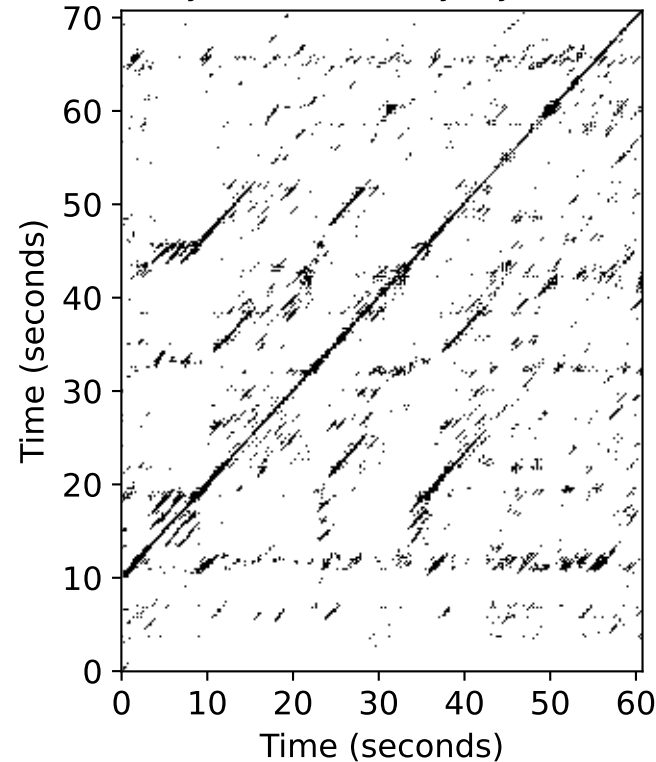
Binary cross-similarity (symmetric)
