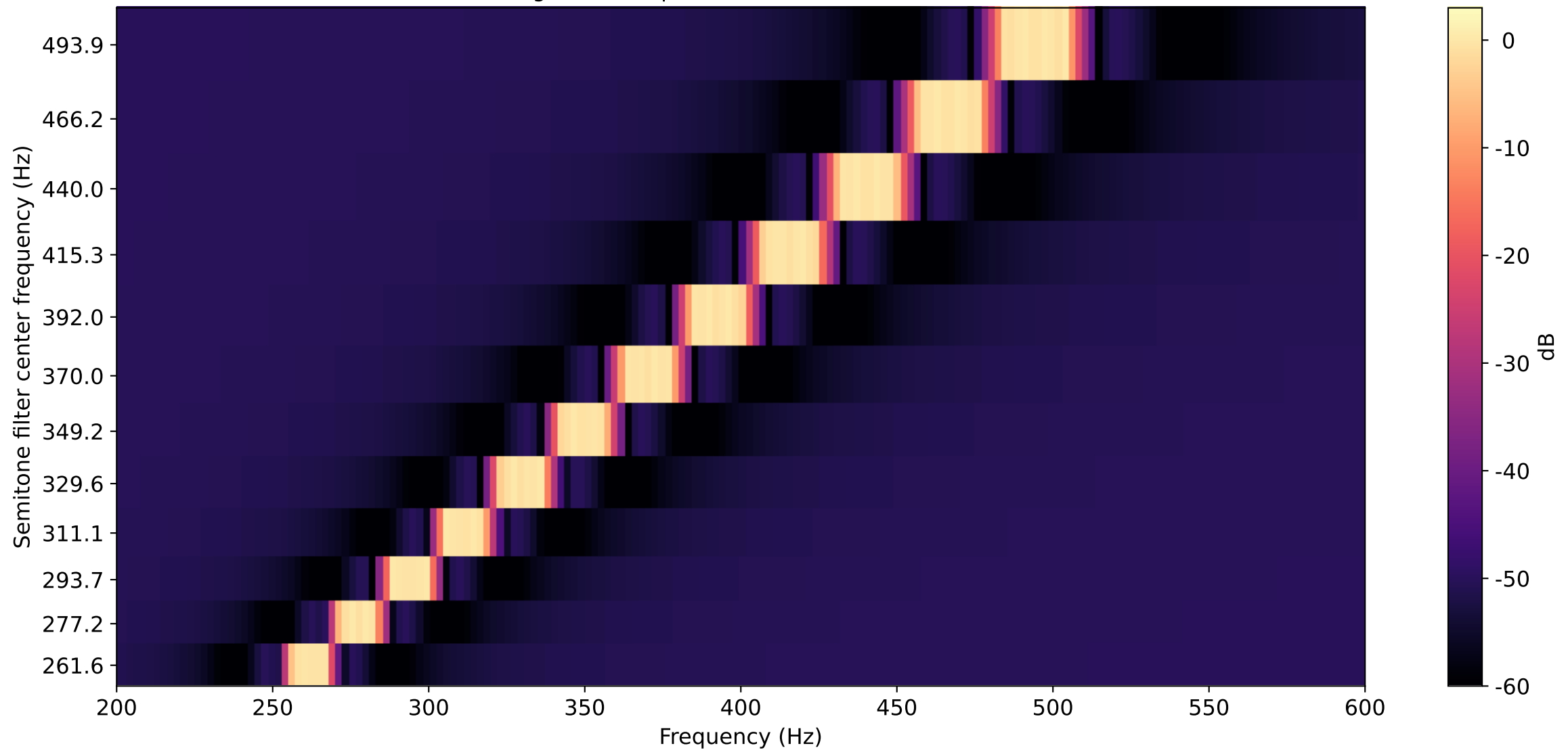
Magnitude Responses of the Pitch Filterbank
