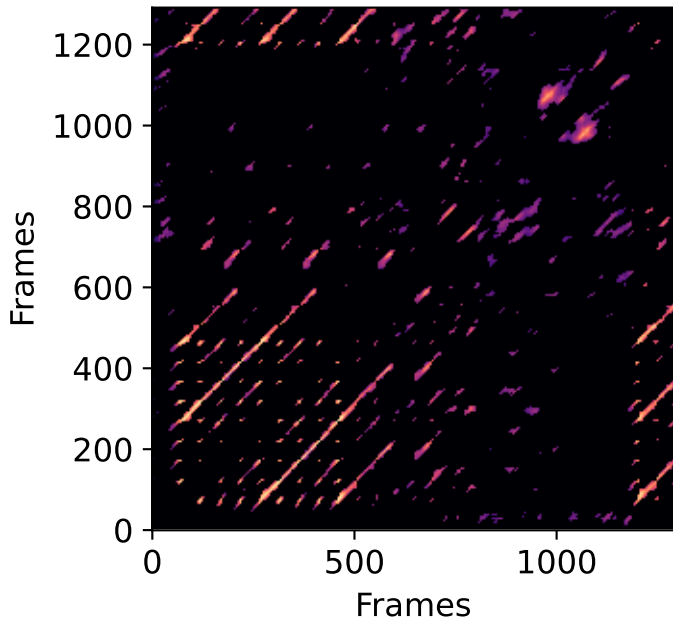
Recurrence matrix
