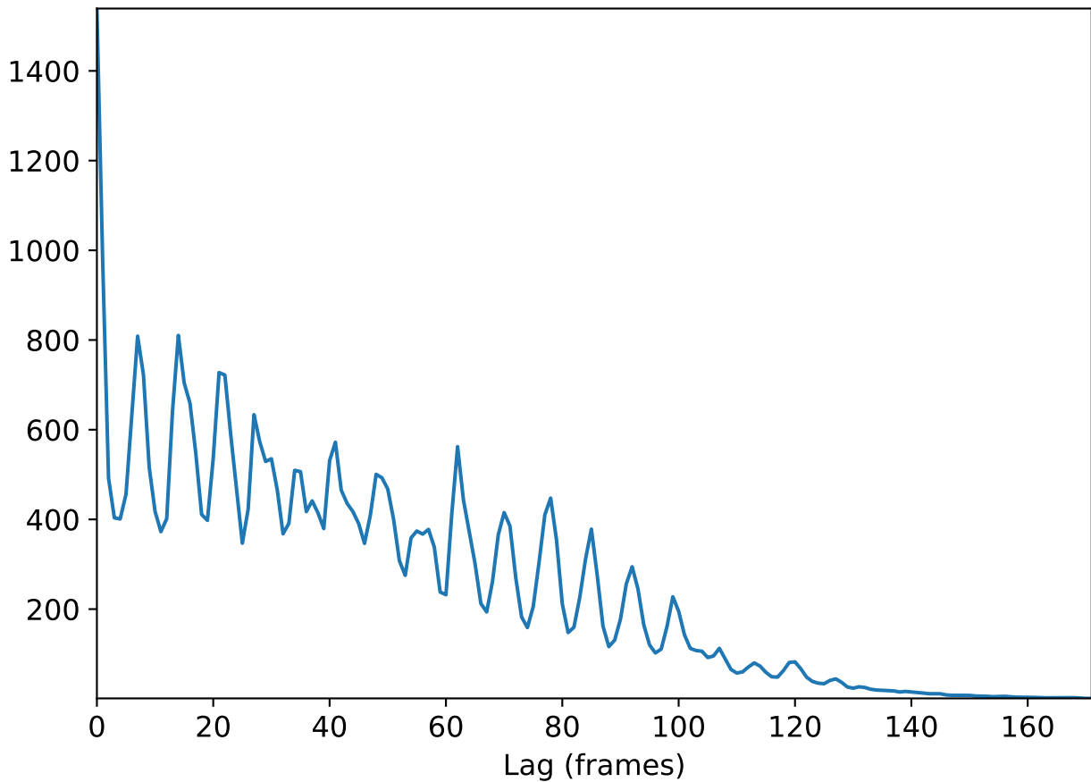
Auto-correlation
